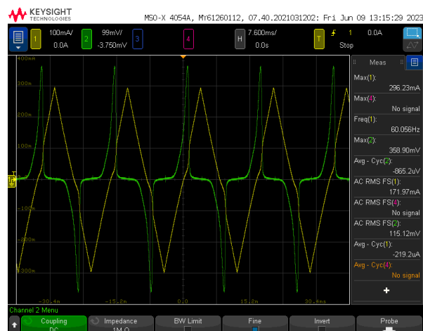
100°C. Sample Triangular Excitation Waveform and B-H Plot. 47 mV pp 60Hz, Amplifier Gain X50.
