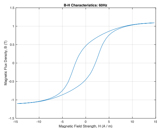
150°C. Sample Sinusoidal Excitation Waveform and B-H Plot. 23.50 mV pp 60Hz, Amplifier Gain X50.
