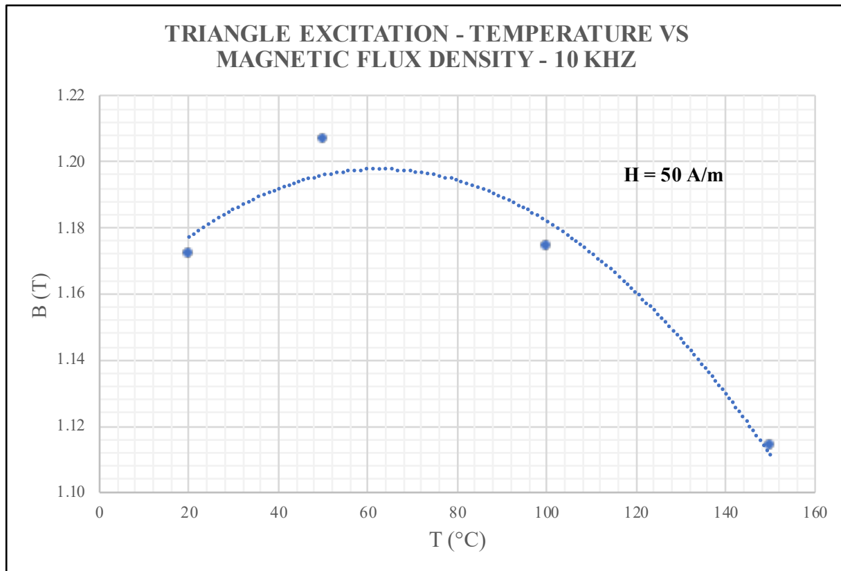
Temperature Dependence vs Core Loss - Table
