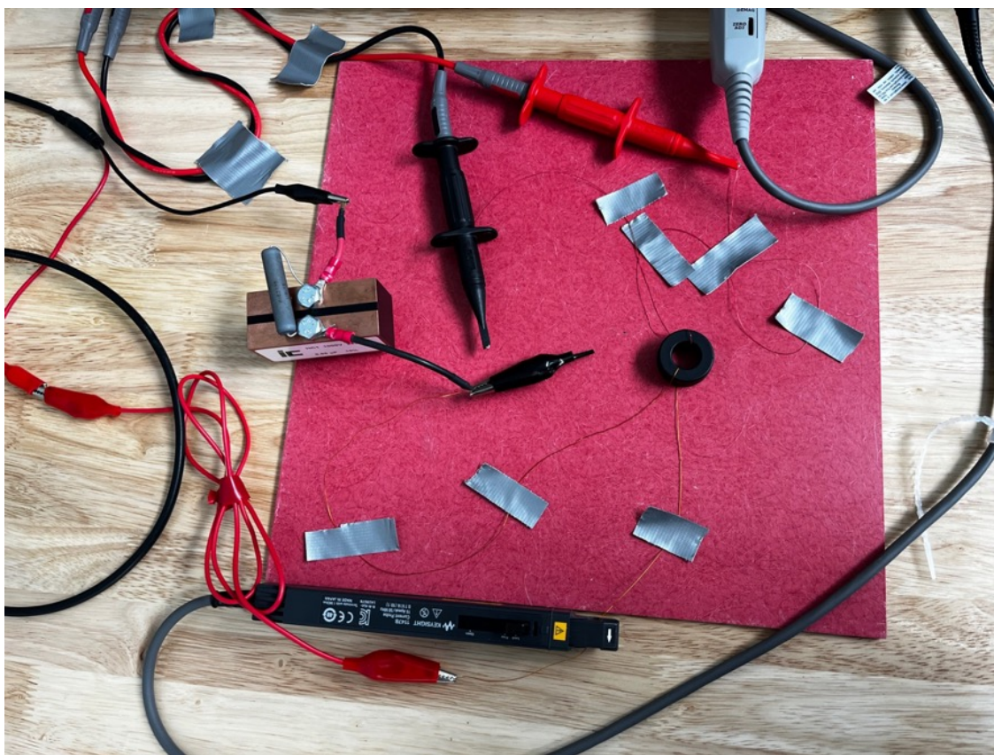
Core Loss Testing - Low Voltage with Amplifier. Cable Layout.
