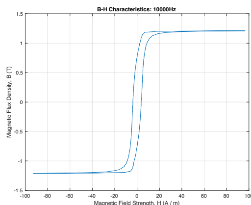
50°C. Sample Square Excitation Waveform and B-H Plot. 234.00 mV pp 10kHz, Amplifier Gain X50.
