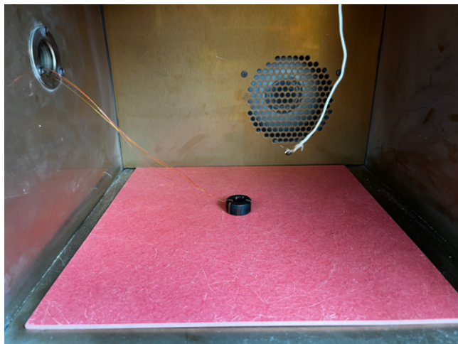
Core Loss Testing - Low Voltage with Amplifier. Typical Test Setup.
