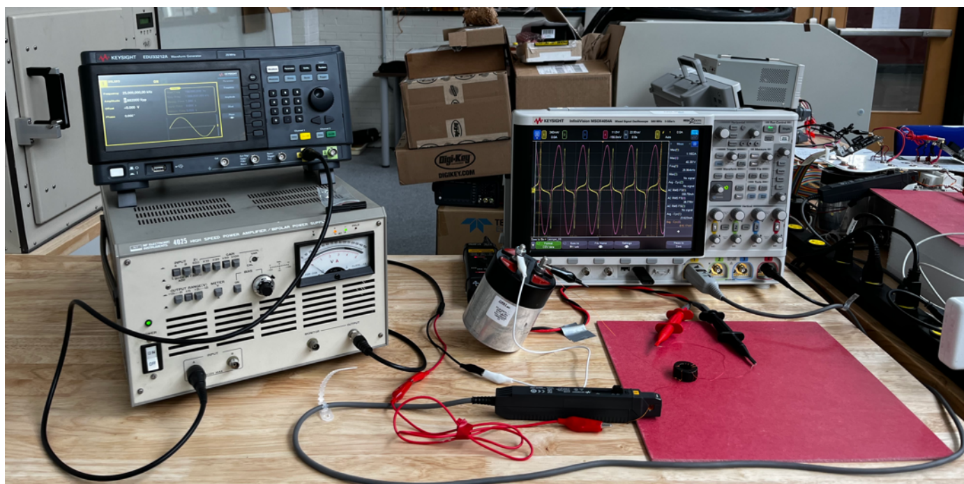
Core Loss Testing - Low Voltage with Amplifier. Typical Test Setup (25 – 200 kHz).
