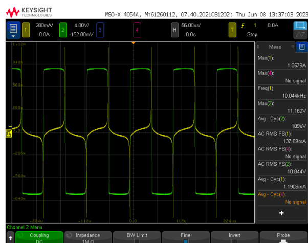
50°C. Sample Square Excitation Waveform and B-H Plot. 234.00 mV pp 10kHz, Amplifier Gain X50.
