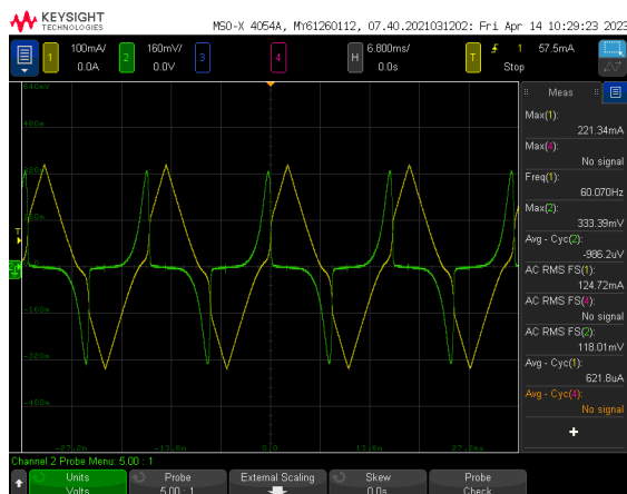
Sample Triangular Excitation Waveform and B-H Plot. Triangular Signal. 27.00 mV pp 60Hz, Amplifier Gain X50.
