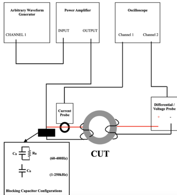
Core Loss Testing - Low Voltage with Amplifier. Typical Test Setup: System Block Diagram.
