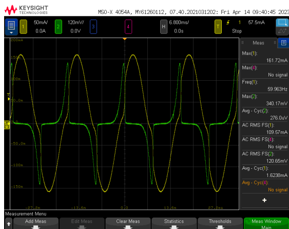
Sample Sinusoidal Excitation Waveform and B-H Plot. Sinusoidal Signal. 19.00 mV pp 60Hz, Amplifier Gain X50.
