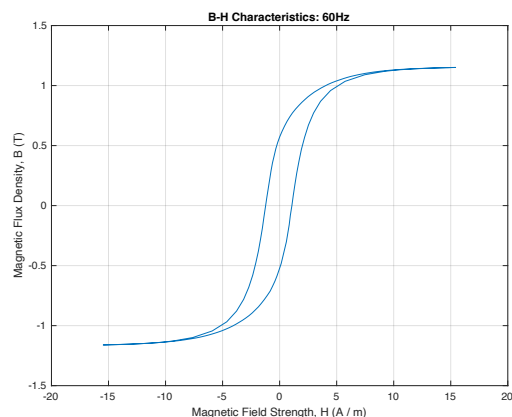
Sample Sinusoidal Excitation Waveform and B-H Plot. Sinusoidal Signal. 19.00 mV pp 60Hz, Amplifier Gain X50.
