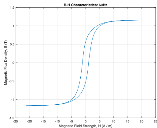
Sample Triangular Excitation Waveform and B-H Plot. Triangular Signal. 27.00 mV pp 60Hz, Amplifier Gain X50.
