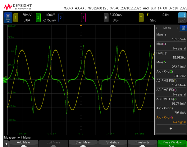
150°C. Sample Sinusoidal Excitation Waveform and B-H Plot. 23.50 mV pp 60Hz, Amplifier Gain X50.
