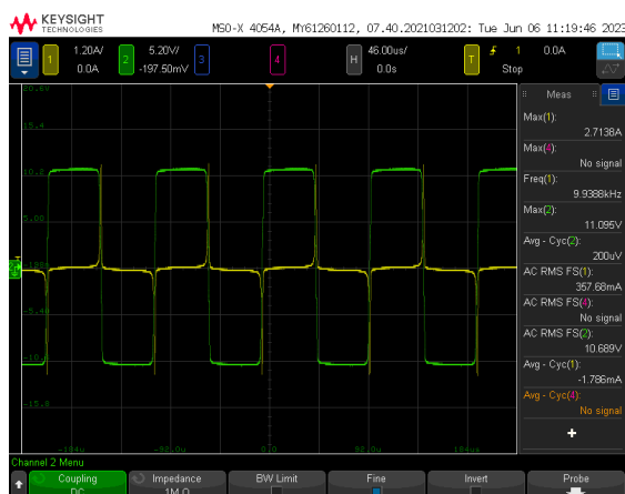
Sample Square Excitation Waveform and B-H Plot. Square Signal. 230.00 mV pp 10kHz, Amplifier Gain X50.
