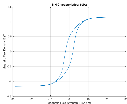
100°C. Sample Triangular Excitation Waveform and B-H Plot. 47 mV pp 60Hz, Amplifier Gain X50.
