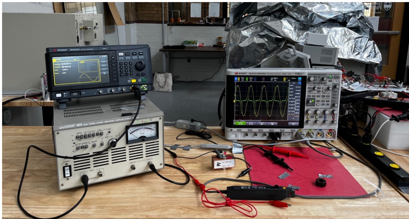
Core Loss Testing - Low Voltage with Amplifier. Typical Test Setup (60 Hz – 10 kHz).
